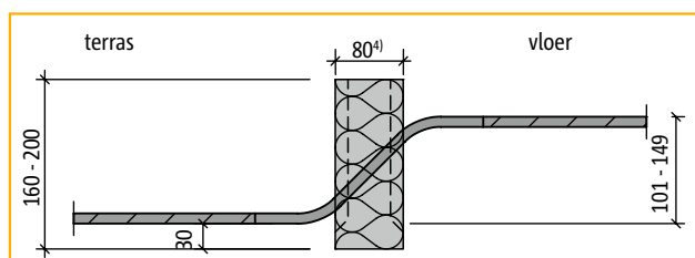
Schöck Isokorb® type QPZ10, QPZ40, QPZ60, QPZ80
